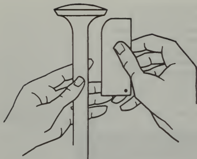
FIGURE 10-5. Checking valve stretch with a manufacturer's gage.
